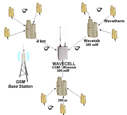
Wavetalk repeaters are often used to forward data via cellular network gateways
